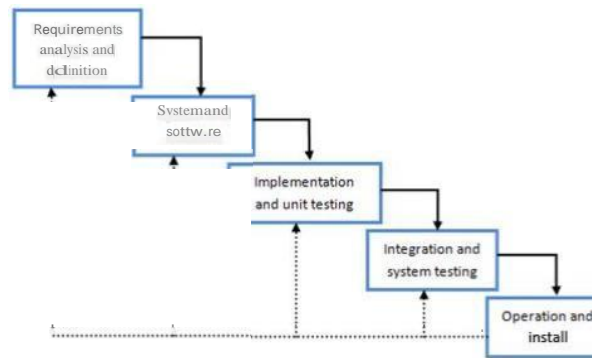
Gambar 1 Model Waterfall Improved
