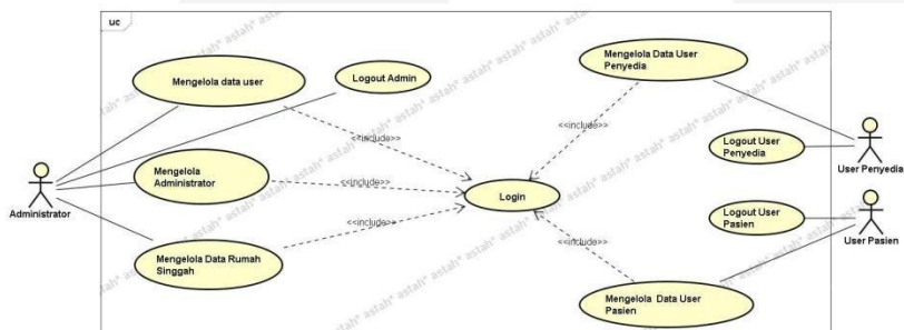
Gambar 5 Diagram Usecase
