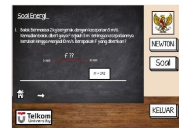
Gambar 3.16 Soal Energi
