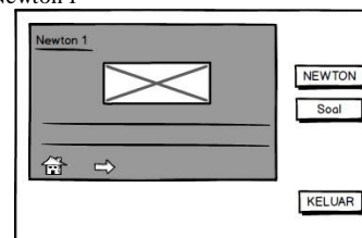
Gambar 1.7 Newton 1
