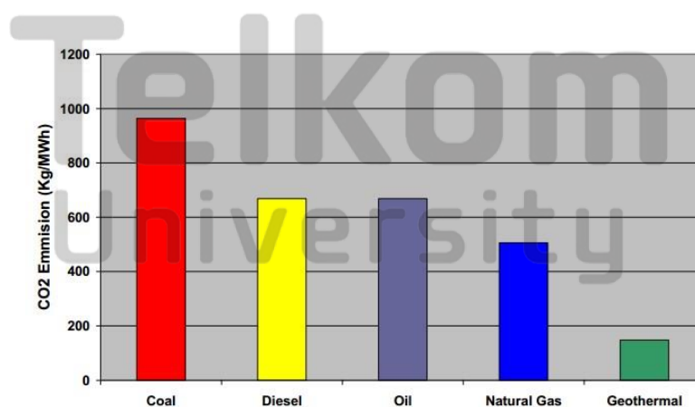
Figure 1.3 The content of emissions generated by some of the energy sources
