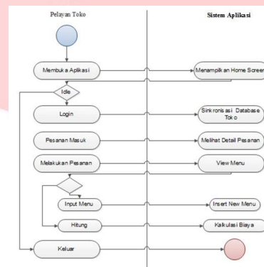
Gambar 2.6 Activity Diagram
