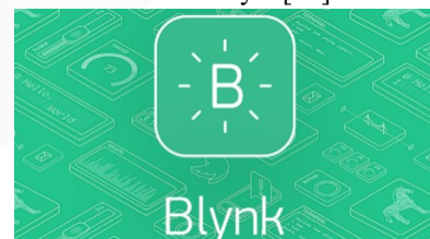
GAMBAR 5 SOFTWARE BLYNK
