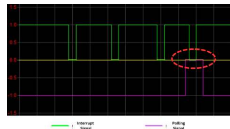
Fig. 4. Signal Output
