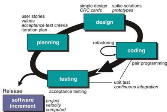
Gambar 1 Extreme Programming
