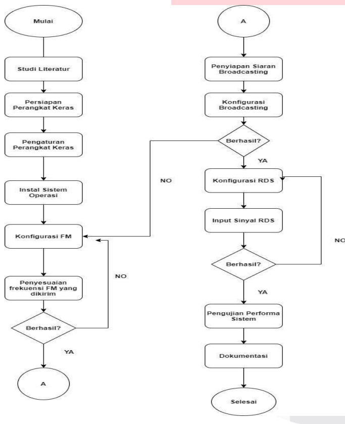
Gambar 3 Flowchart
