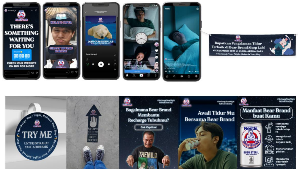
Gambar 3 Media Interest
