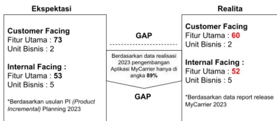
Gambar 1.1 Analisis Gap
