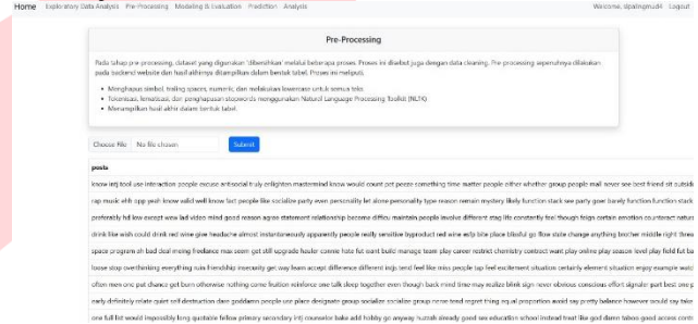
Gambar 10. Tahap Pre-Processing
