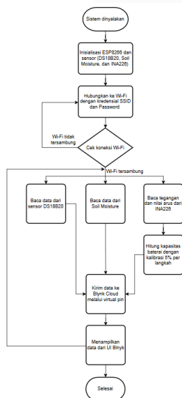
Gambar 3. Flowchart alur sistem IoT
