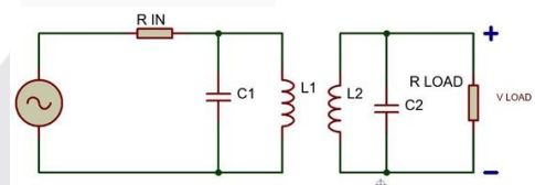
Gambar 1. Skematik coil .
