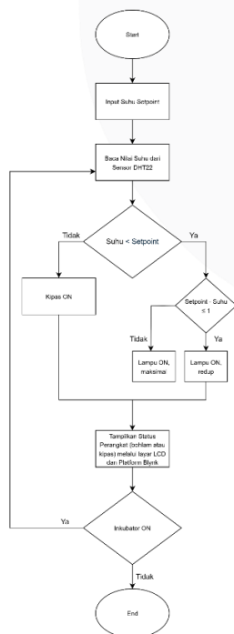
GAMBAR 6 FLOWCHART
