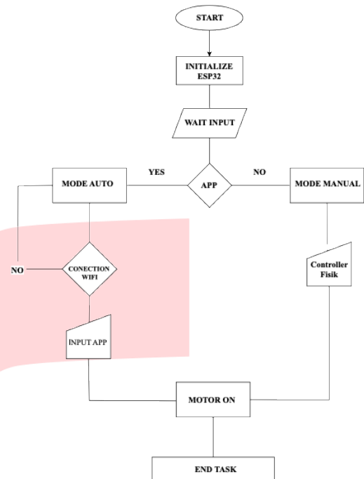
Gambar 3.4 Flowchart sistem
