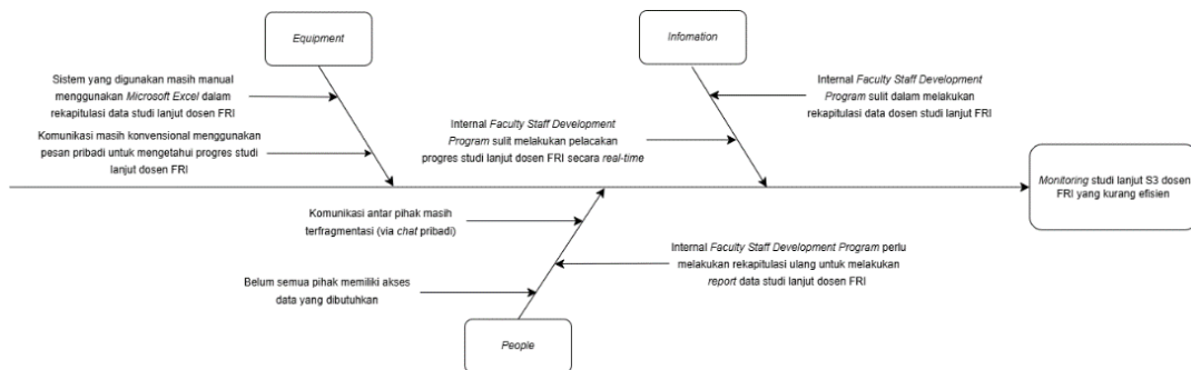
Gambar I. 1 Diagram Fishbone
