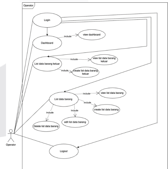
Gambar 6 Use case diagram operator
