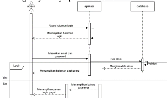
Gambar 8 Sequence Diagram
