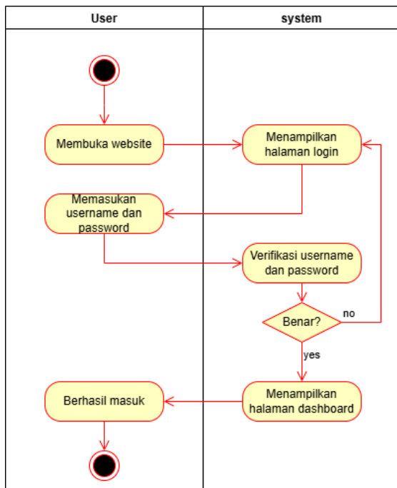
Gambar 7 Activity diagram
