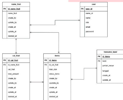
Gambar 4 Entity relation diagram.
