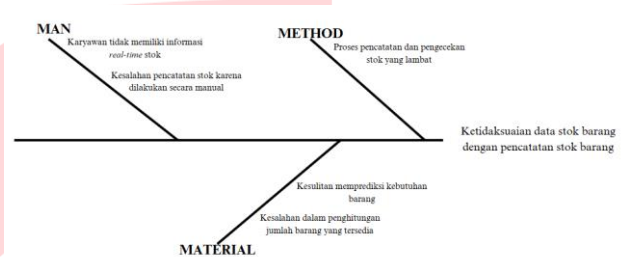
Gambar I Fishbone.
