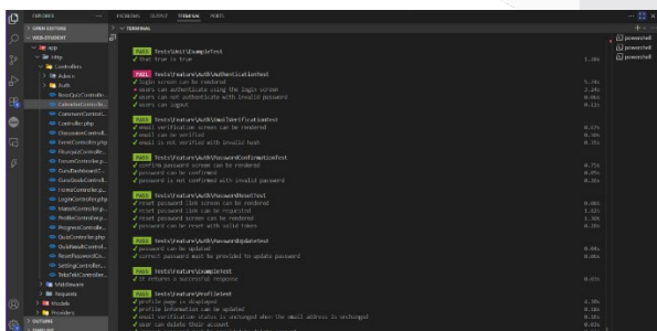
Gambar 3 Whitebox Testing
