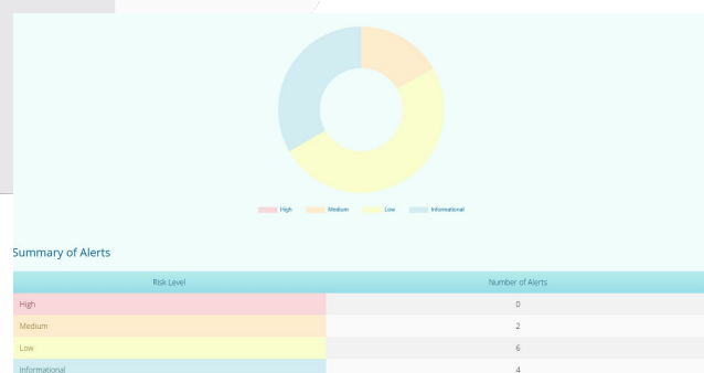
Gambar 4 Security Testing
