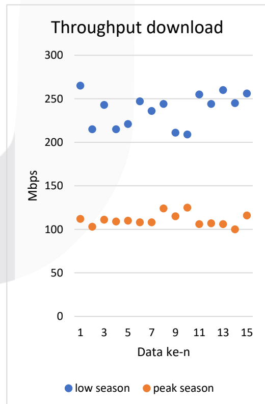
GAMBAR 9 (GRAFIK DOWNLOAD THROUGHPUT)
