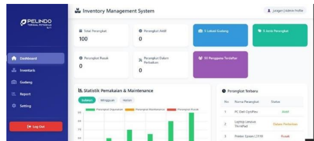
Gambar 9 Dashboard
