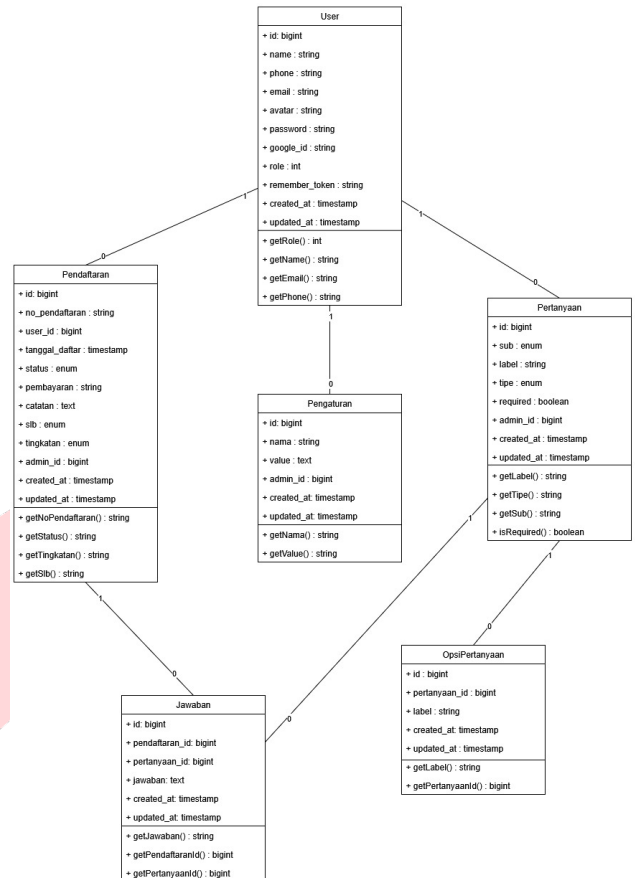
Gambar 4. Class Diagram
