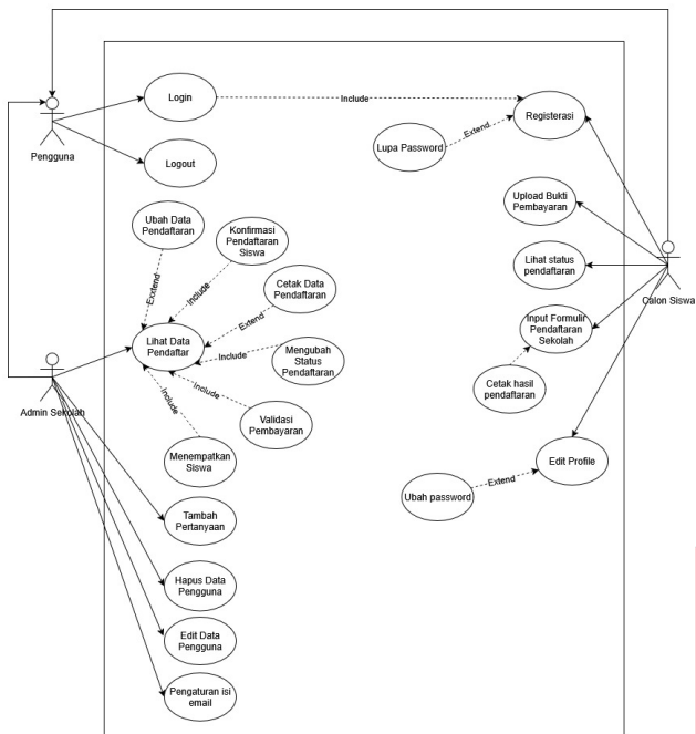
Gambar 2. Usecase Diagram
