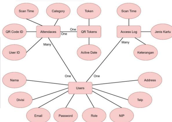
Gambar 4 Diagram Entity Relationship (ERD)
