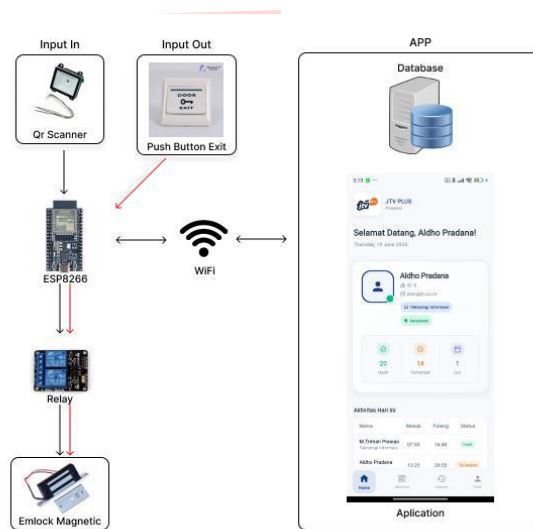
Gambar 3 Blok Diagram
