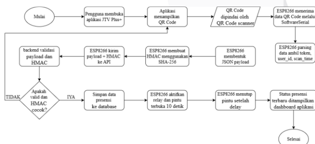
Gambar 2 Flowchart Sistem Presensi
