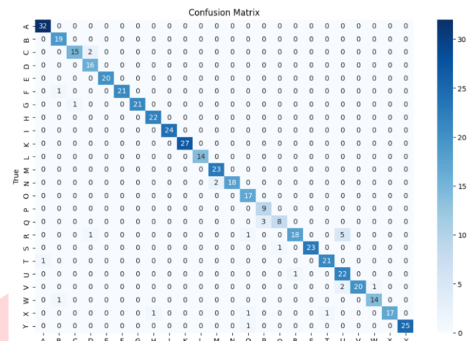
Gambar 10 Confusion Matrix
