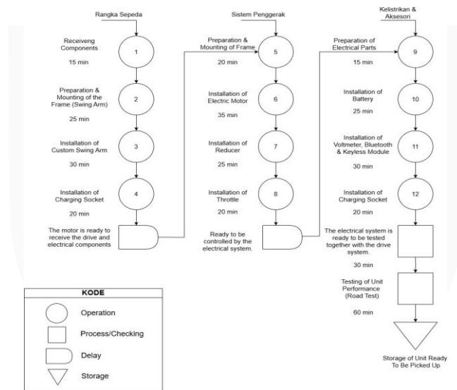
Gambar 5. Operation Process Chart (OPC)
