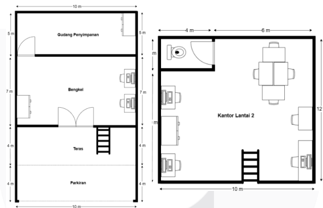
Gambar 3. Layout Bengkel
