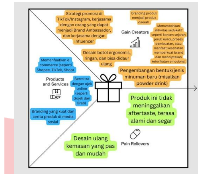
Gambar 4.3 Value Map
