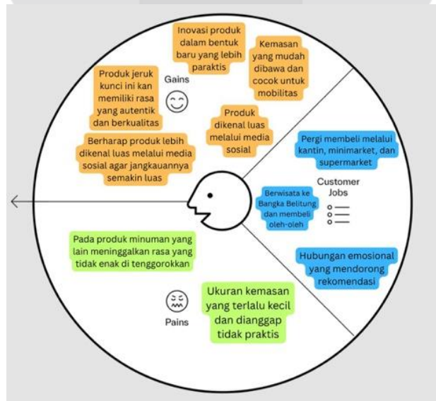
Gambar 4.2 Customer Profile
