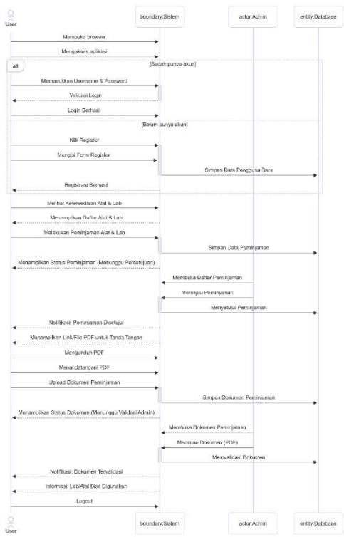
GAMBAR 6 (SEQUENCE DIAGRAM)
