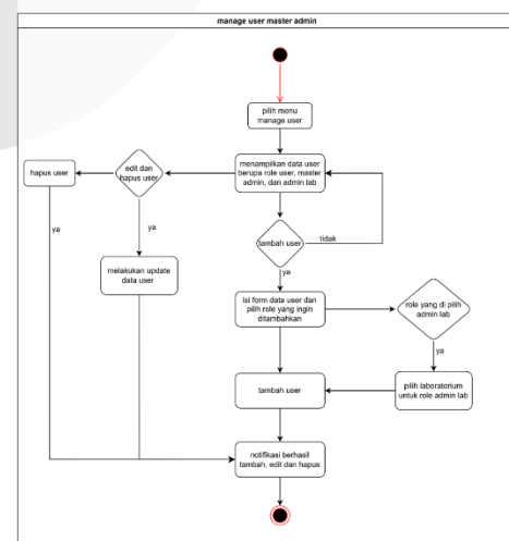
GAMBAR 5 (ACTIVITY DIAGRAM)
