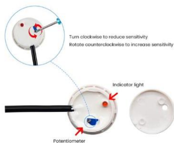
Gambar 1 Sensor Non-contact Liquid
