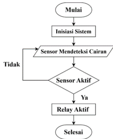
Gambar 2 Flowchart Sistem Alat
