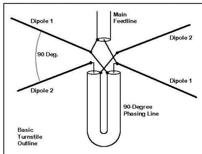
Gambar 1 Antenna turnstile
