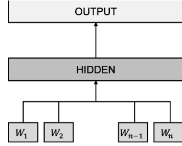
Fig. 1. FastText Architecture [15].
