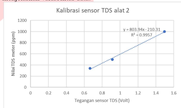
Gambar 12. Kalibrasi Sensor TDS SEN0244 Alat 2
