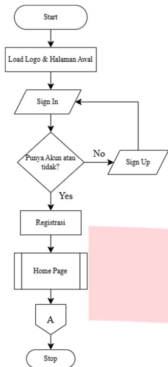
Gambar 4. Flowchart Mobile Application
