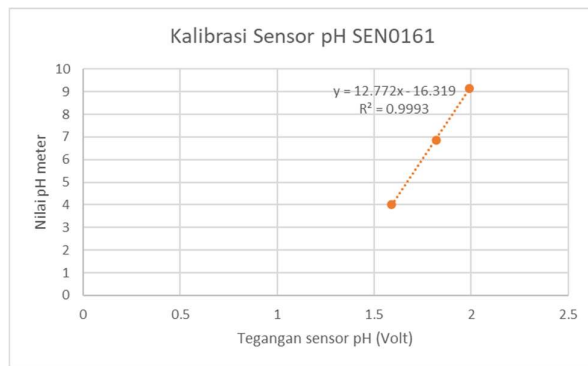
Gambar 10. Kalibrasi Sensor pH SEN0161
