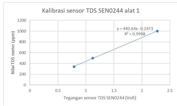
Gambar 11. Kalibrasi Sensor TDS SEN0244 Alat 1
