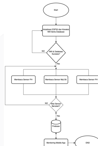
Gambar 3. 1 Flowcard Sistem
