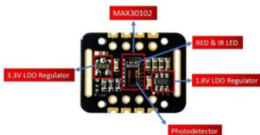
GAMBAR 2 (SENSOR MAX30102)[5]
