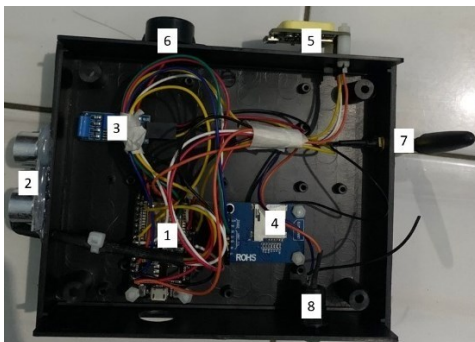
GAMBAR 7 Perancangan Hardware
