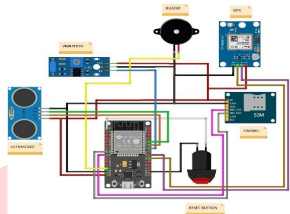
GAMBAR 5 Perancangan Hardware
