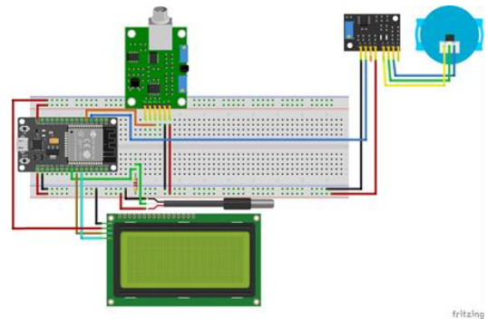
GAMBAR 10 (Sirkuit Diagram)
