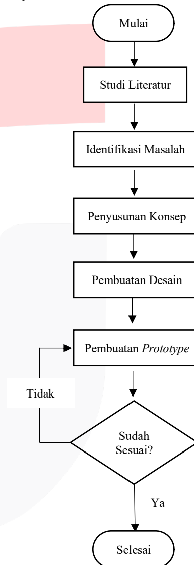
Gambar 1. Alur Penelitian
