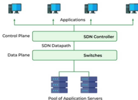
Gambar II.2 Software Defined Network
