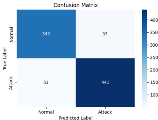
Gambar V.3.1 Confusion Matrix
