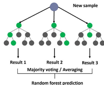
Gambar II.4 Random Forest
