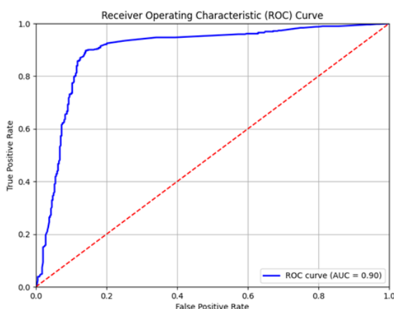
Gambar V.4.1 ROC Curve
