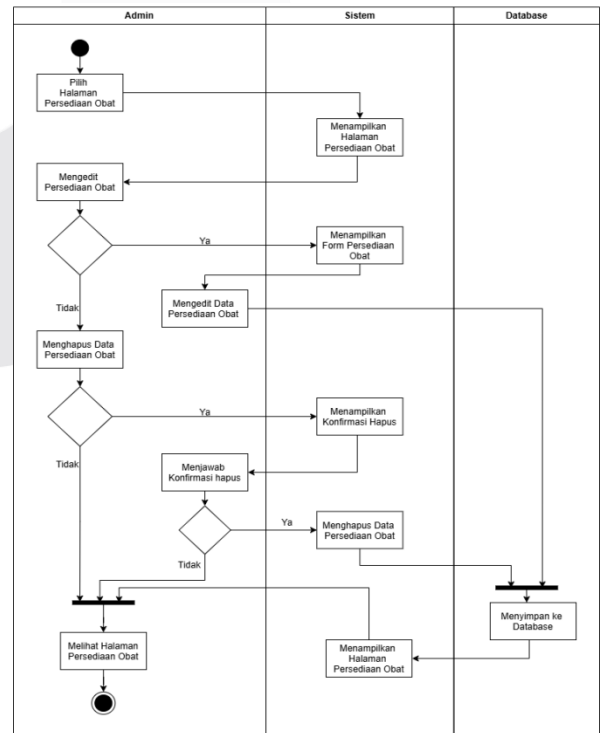
GAMBAR 11 (Activity Diagram Halaman Persediaan Obat)
