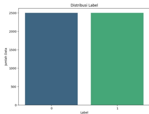
Gambar 5. Distribusi Dataset
