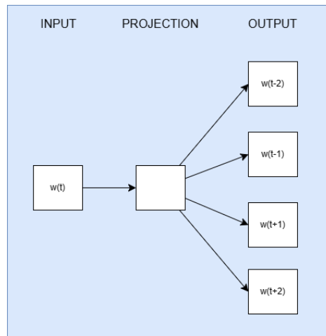
Gambar 3. Tahapan Skip-gram
