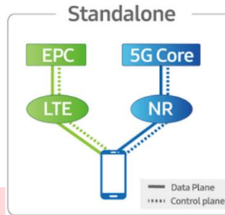
GAMBAR 2 (STANDALONE)
