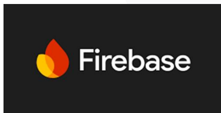
GAMBAR 14 (FIREBASE [17])
