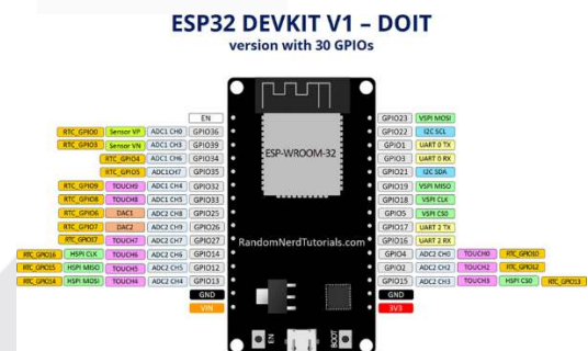
GAMBAR 3 (PIN OUT ESP32 [6])
