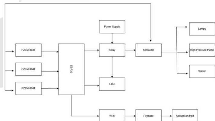
GAMBAR 16 (DIAGRAM BLOK)
