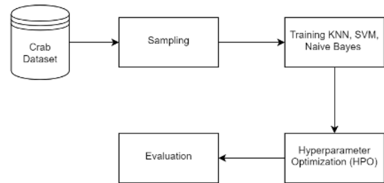
Fig. 3. Proposed Method
