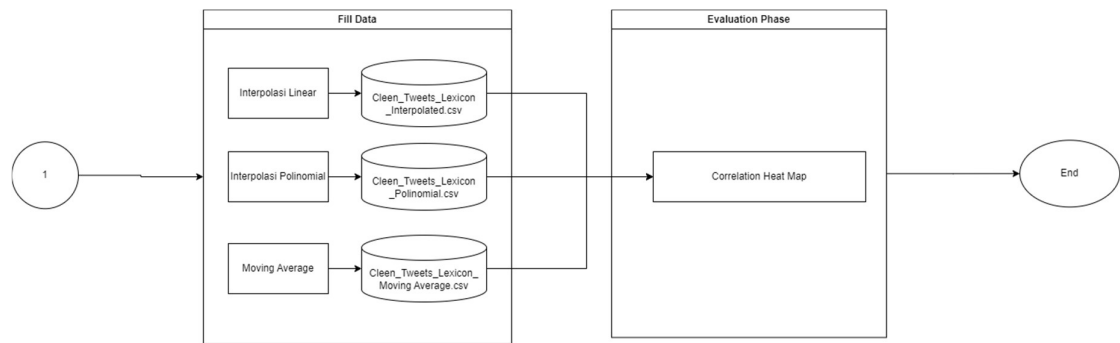
Gambar 3.2 Flowchart
