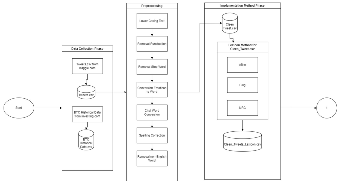
Gambar 3.1 Flowchart
