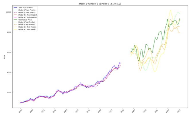
Gambar 5. Prediksi Saham BBCA
