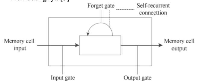
Gambar 1. LSTM Model Memory Cell
