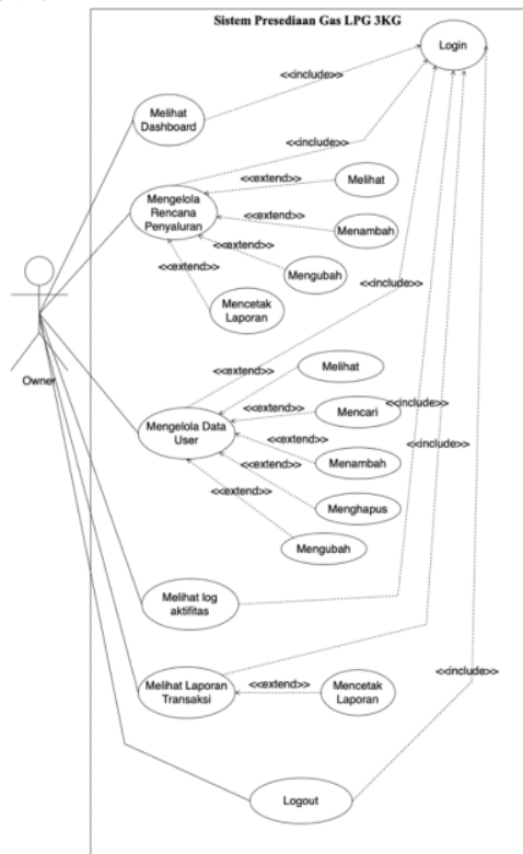
Gambar 5 (Usecase Diagram Owner)
