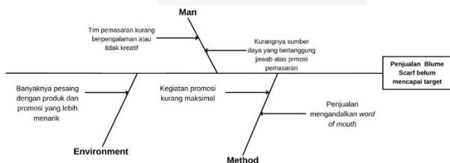
GAMBAR 4 Fishbone
