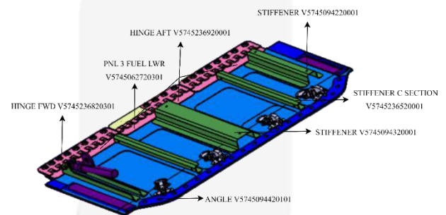
Gambar 1 Komponen Panel 3 Fuel Lower
