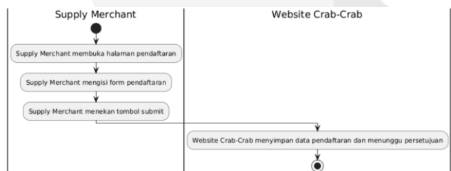
Gambar IV.6 Activity Diagram Register Supply Merchant
