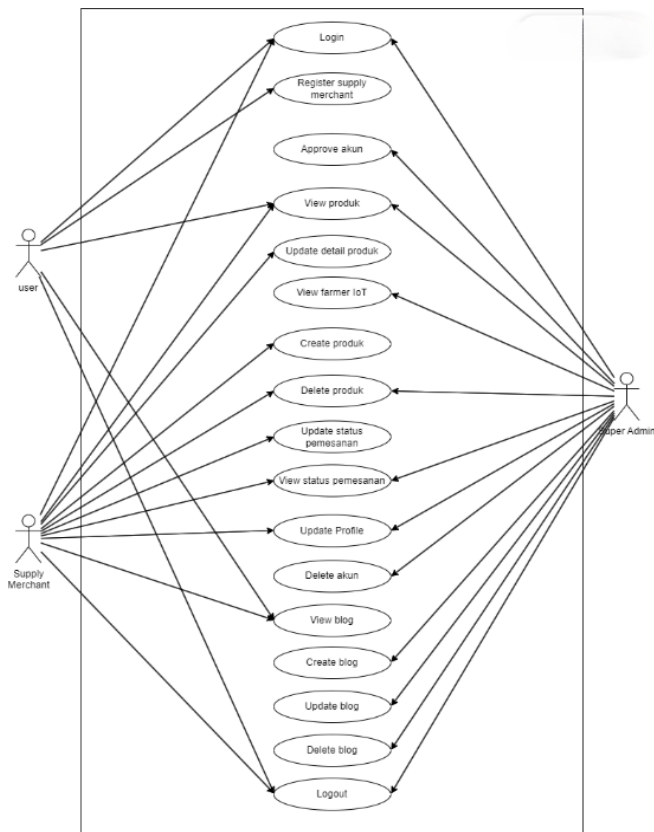
Gambar IV.4 Use Case Diagram
