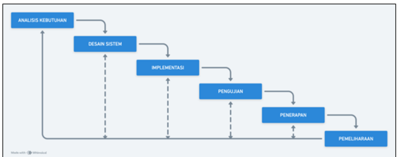
Gambar 1.1 Metodologi Waterfall
