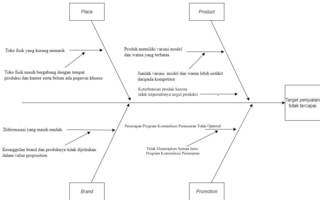
Gambar I. 4 Diagram Fishbone
