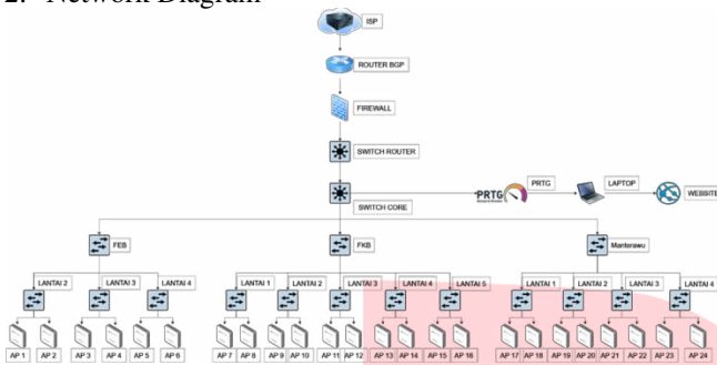
GAMBAR 1 Network Diagram
